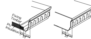
Profile of Gutter Version Profile of Solid Version
